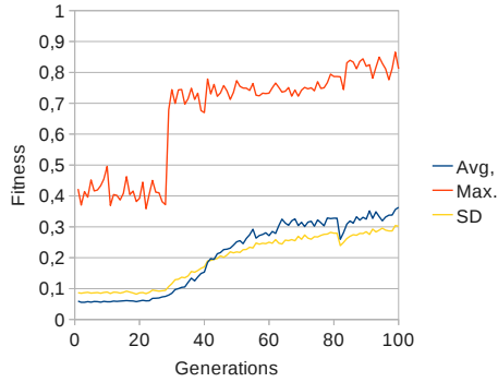
Fig. 3. Average and maximum fitness during an evolutionary run.
