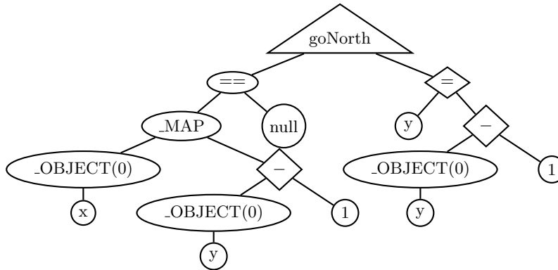
(b) A simple Go North example
